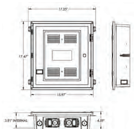
Narrow lid lowers profile 1 inch
