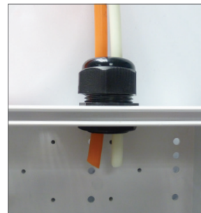
Upward facing installation
