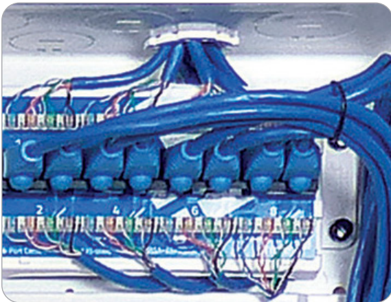
Cable ties can be used to secure cabling in media panels
