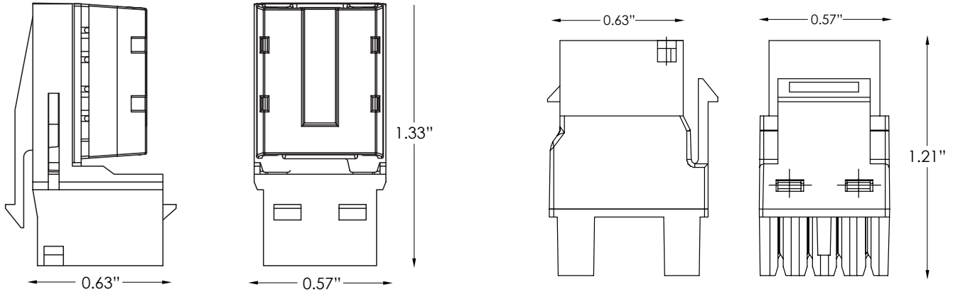
Cat6 90° Keystone
