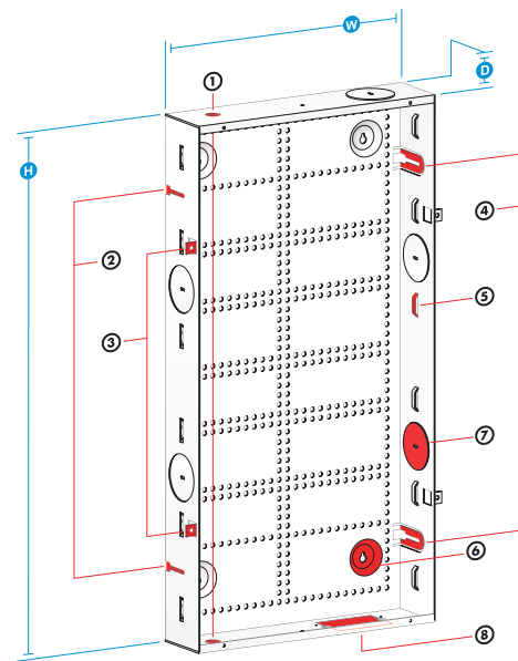
SMS Shelf Mounting System (Sold separately)
