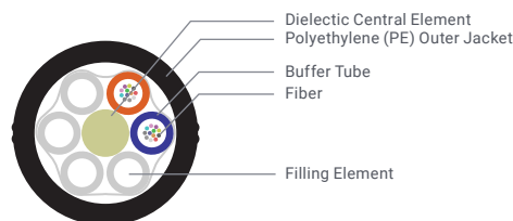
Round Cable* Construction
